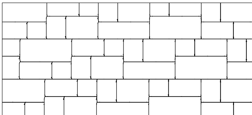
ASHLAR INSTALLATION PATTERN: 6" Units (43%), 8" Units (57%)
